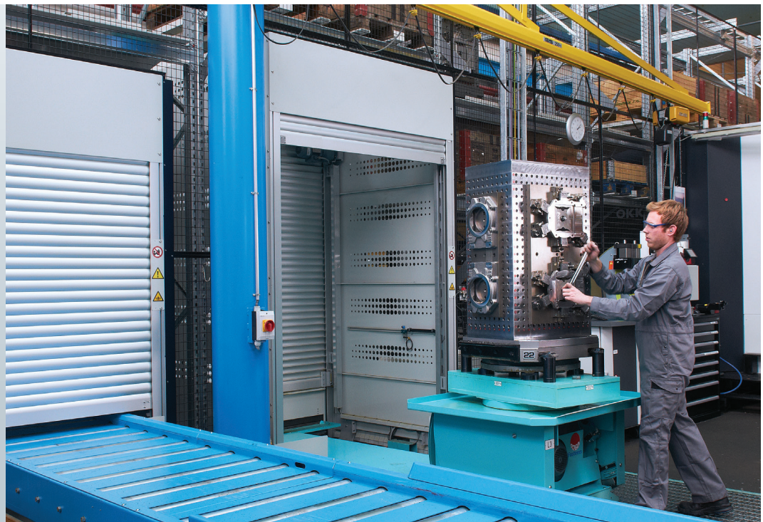
Flexible manufacturing system with intergrated material management
