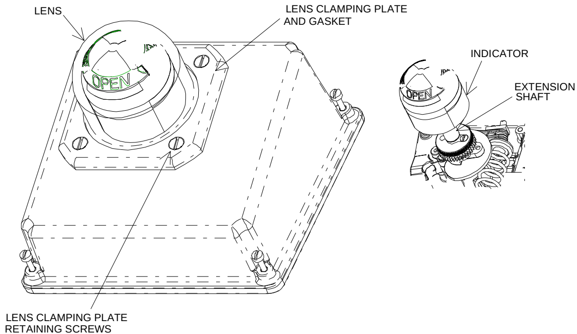
FIGURE 4-8 Beacon Indicator
