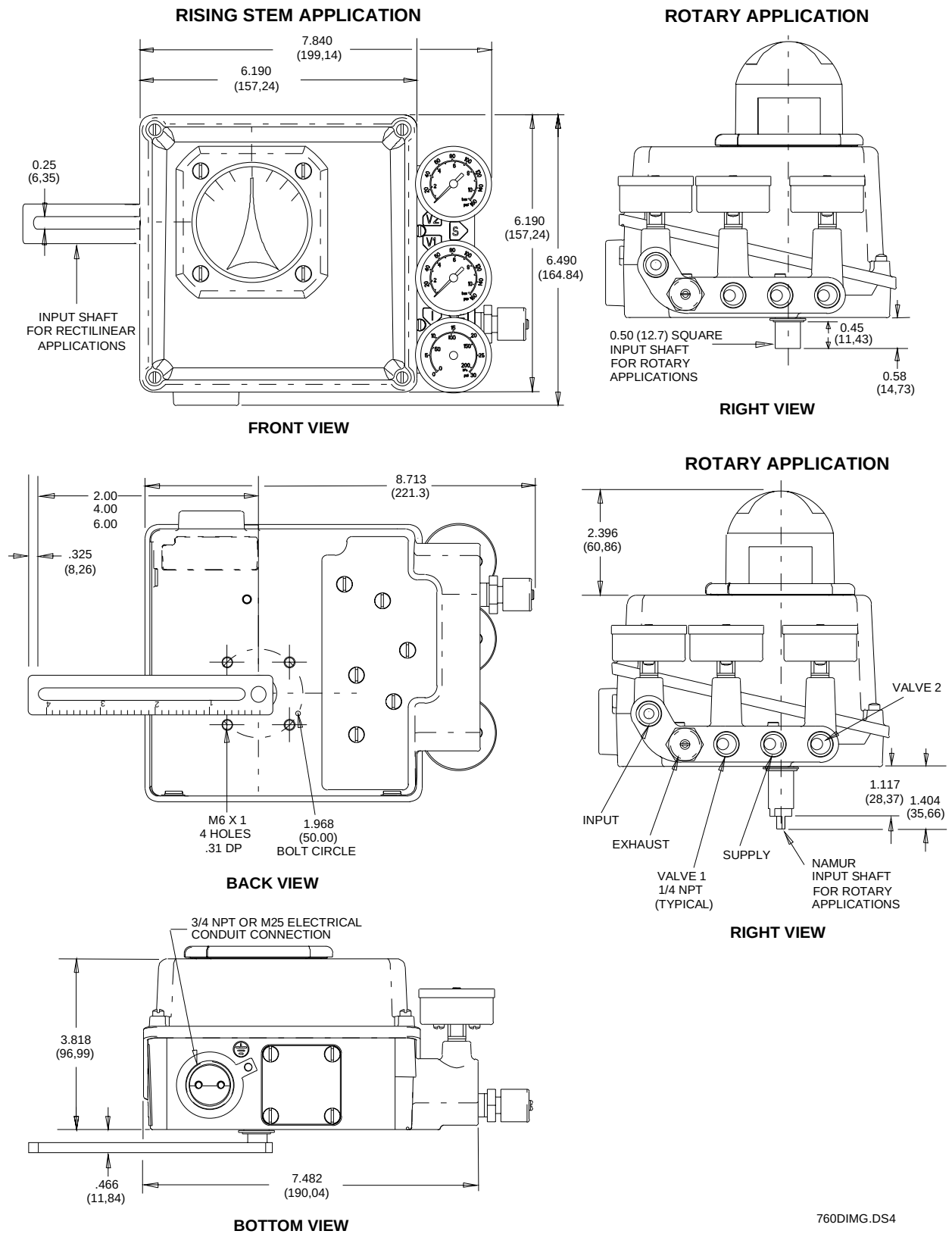
FIGURE 2-1 Installation Dimensions
