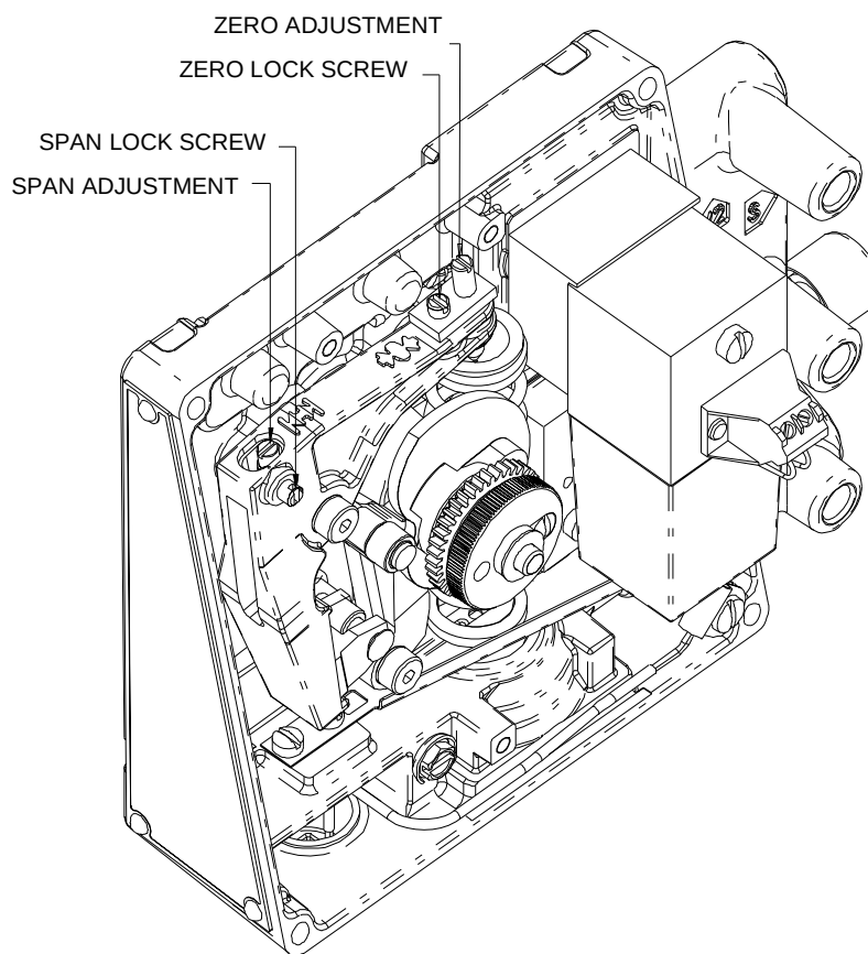
FIGURE 3-3 Calibration Adjustments
